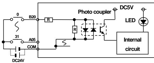
Circuit configuration
